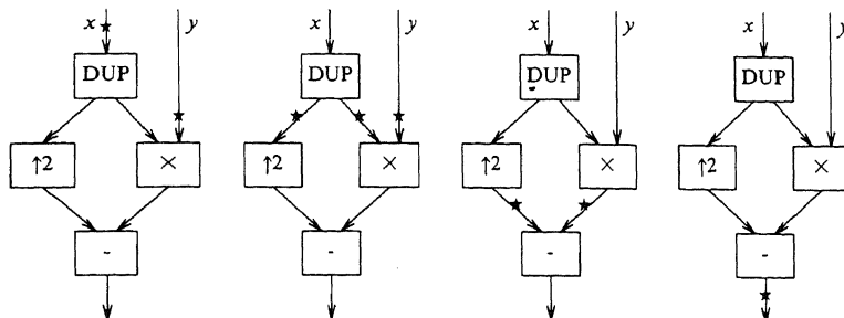
Figure 3. An execution sequence
