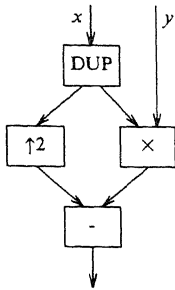
Figure 2. A dataflow graph
