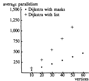
Figure 11. Performance on the dataflow machine. (a) Total number instructions; (b) Critical path length; (c) Average parallelism
