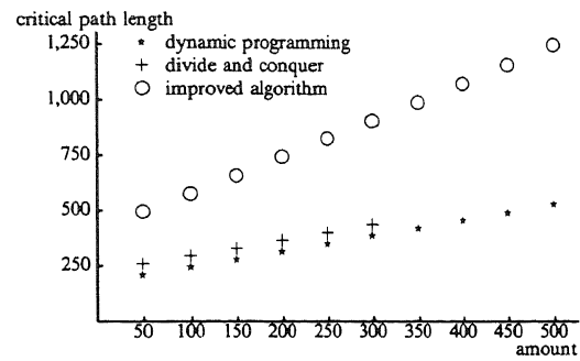
Figure 8. Critical path length on the dataflow machine
