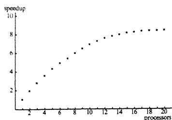
Figure 12. Typical speedup curve for dynamic programming on the dataflow machine; n = 40 and b = 300
