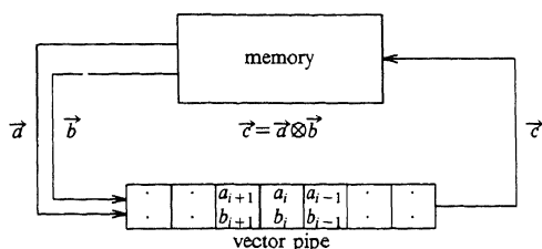
Figure 5. The CYBER-205
