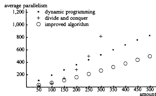
Figure 9. Average parallelism on the dataflow machine
