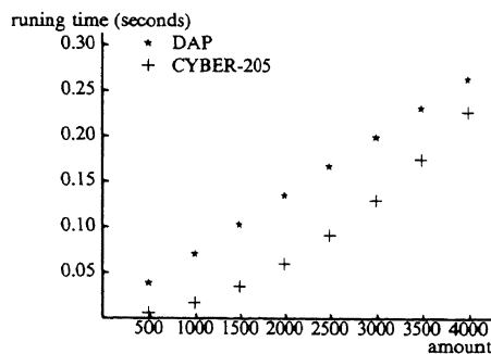
Figure 10. Dynamic programming on the DAP and CYBER-205
