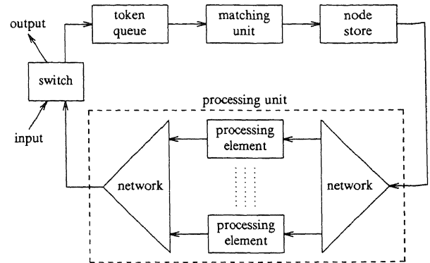
Figure 4. The Manchester dataflow machine
